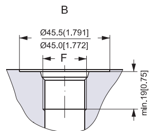
B: UN main ports F: 1 5/16 - 12 UN O-ring boss port
